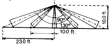
Ceiling Mount 360°
